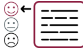
SENTIMENT CLASSIFIER
